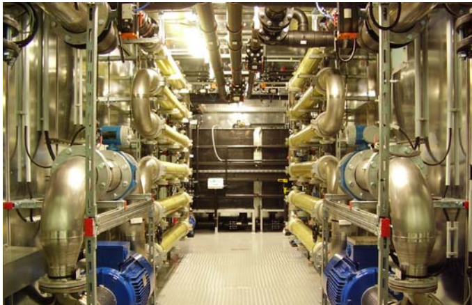
Figure 5 Compact MBR Container
