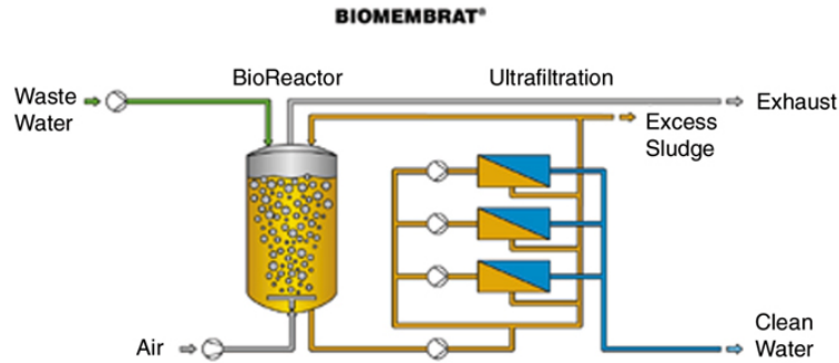
Figure 1 MBR Flow Diagram
