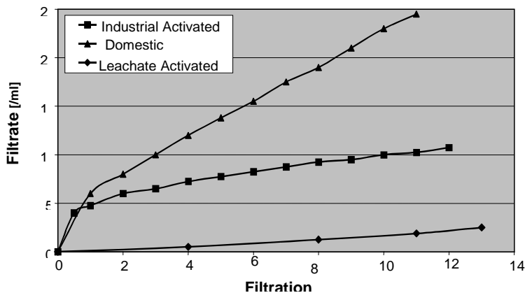
Figure 6 Filterability Comparison
