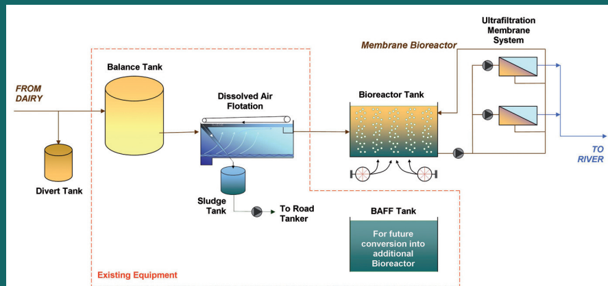
Figure 2 Wehrle Process Flow Diagram
